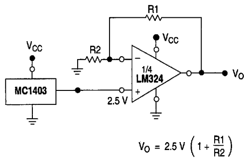
Figure 7. Voltage Reference
