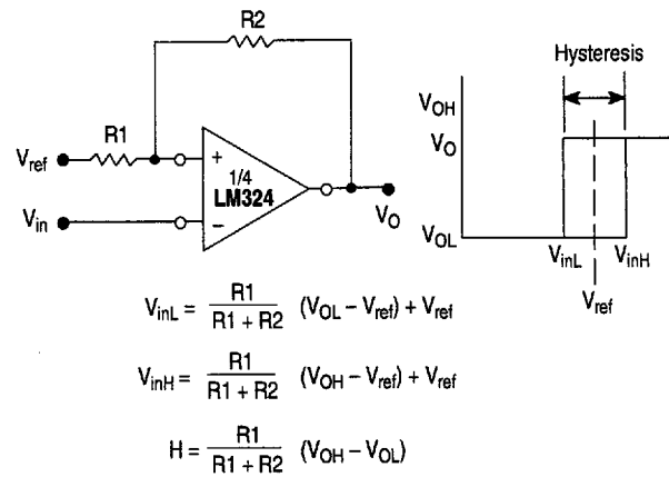
Figure 10. Comparator with Hysteresis
