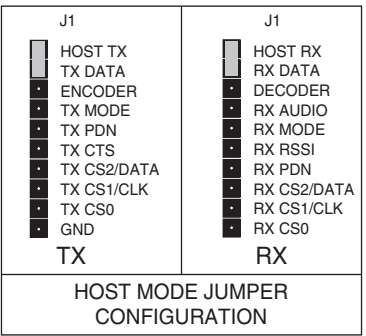
Figure 5: Jumper Configuration
