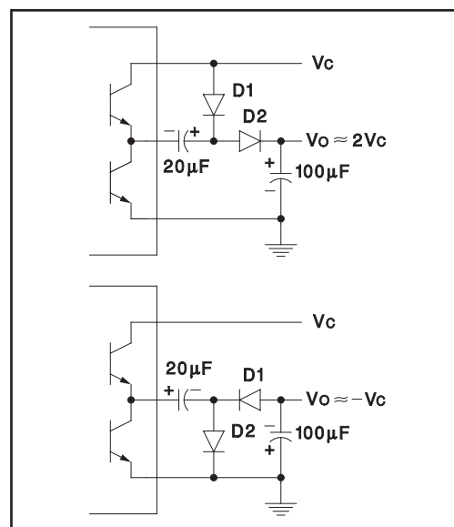
Charge Pump Circuits
