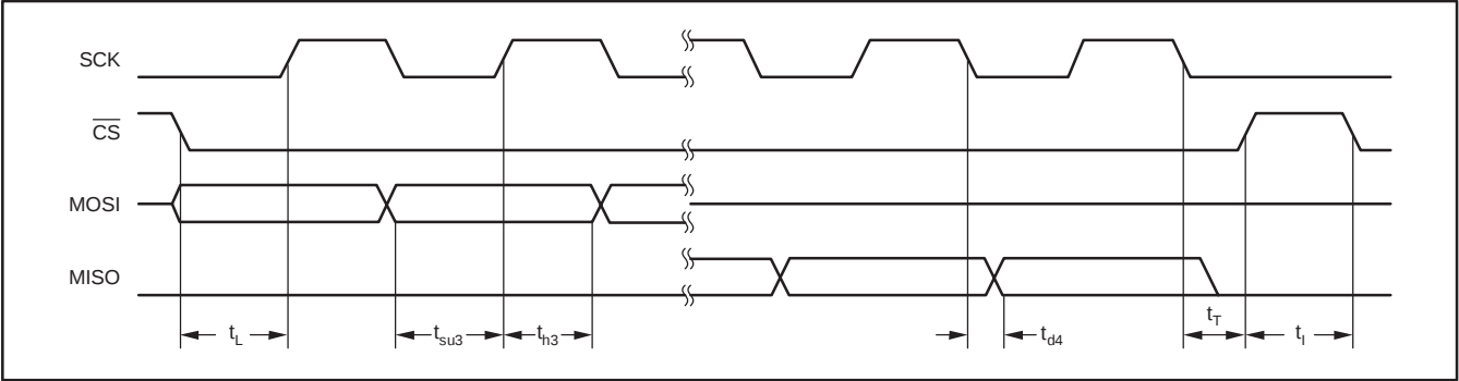
Figure 3. Control Interface Timing
