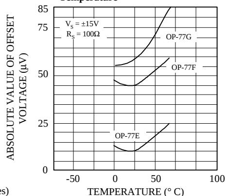
Untrimmed Offset Voltage vs Temperature
