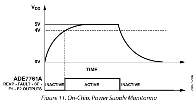
Figure 11. On-Chip, Power Supply Monitoring
