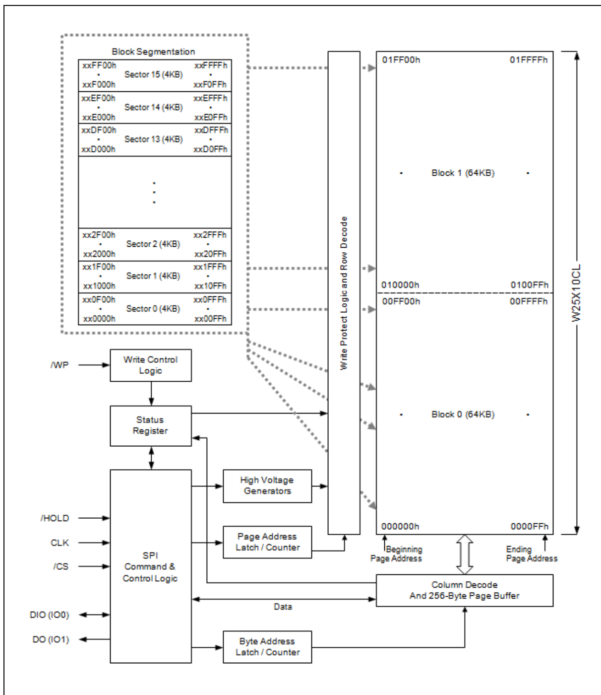
Figure 2. W25X10CL Serial Flash Memory Block Diagram
