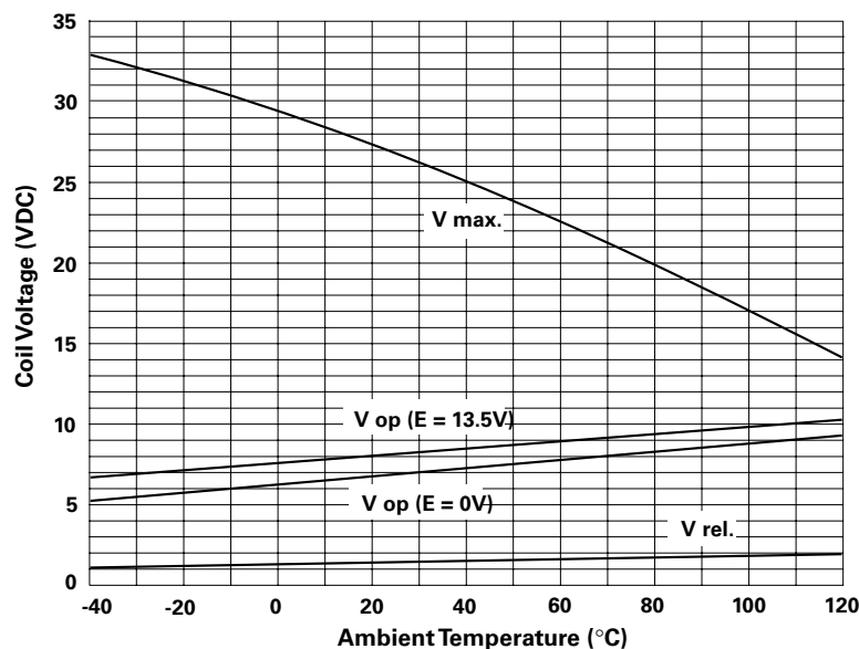
Figure 1 - Operating Voltage Range
