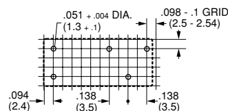
8/12A, 5 mm Pin Spacing
