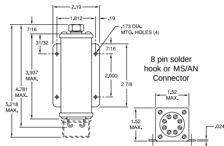
Panel Mount —H1, —H3
