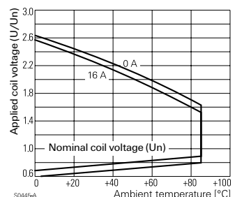
410 83 Type 1 Form X, 3 mm Contact Gap
