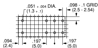
16A, 5 mm Pin Spacing
