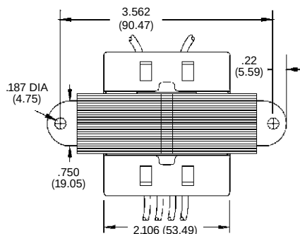
Type K Foot Mount 60VA
