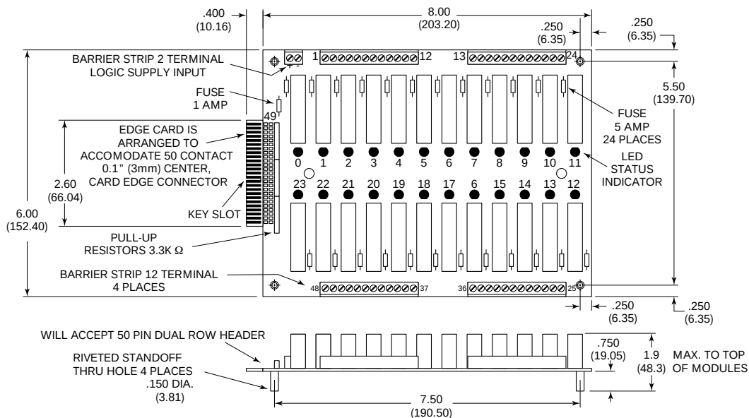
2IOM24D With Straight Header
