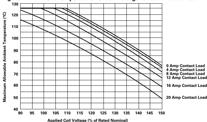
Figure 2 – Ambient Temperature vs. Coil Voltage for Continuous Load
