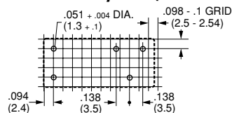
8/12A, 3.5 mm Pin Spacing
