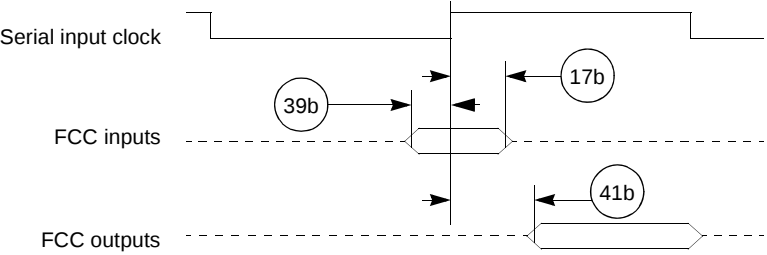
Figure 2-19. FCC External Clock Diagram
