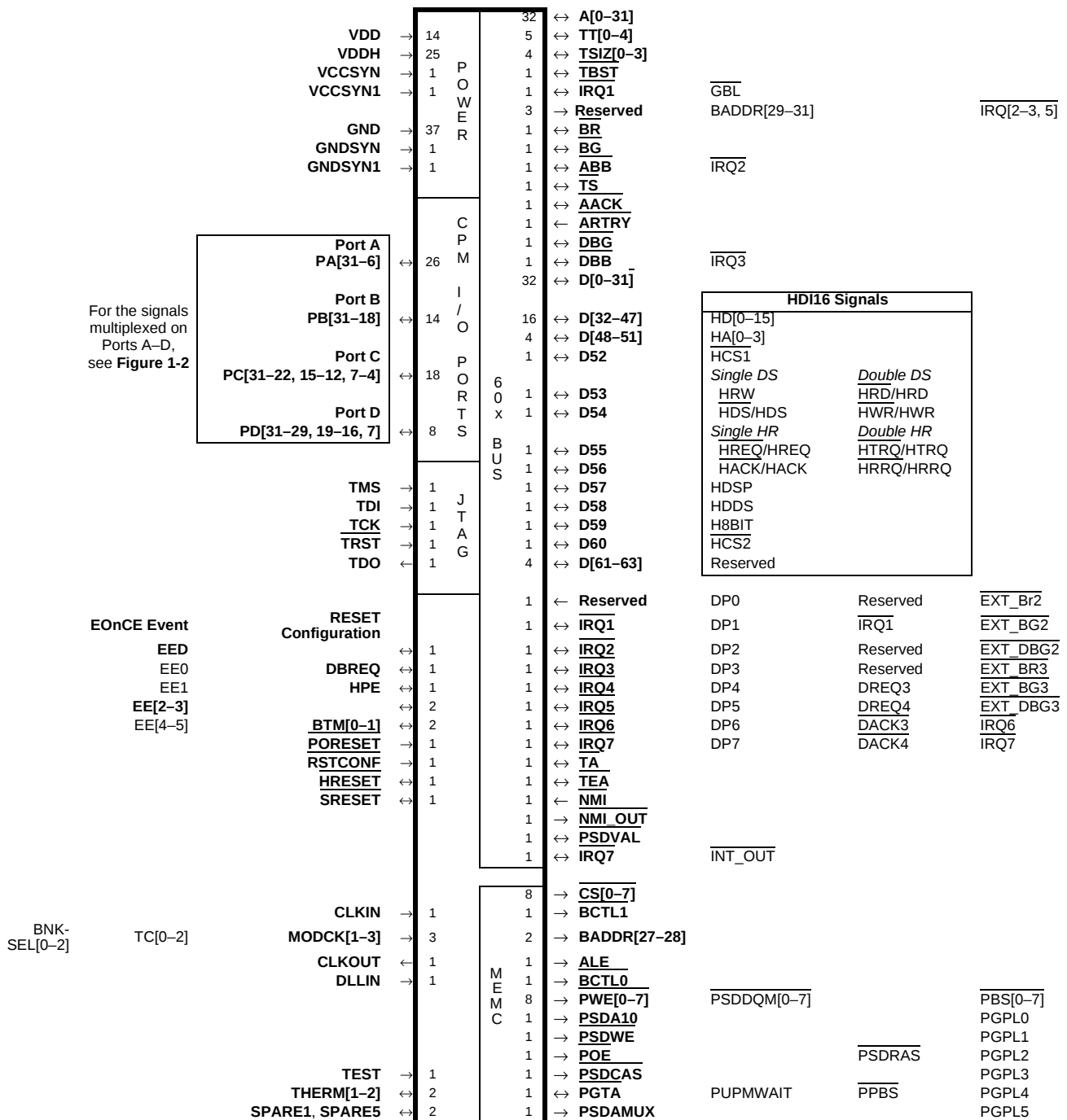
Figure 1-1. MSC8103 External Signals
