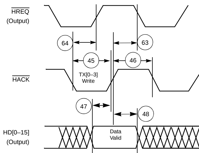
Figure 2-17. Host DMA Write Timing Diagram, HPCR[OAD] = 0
