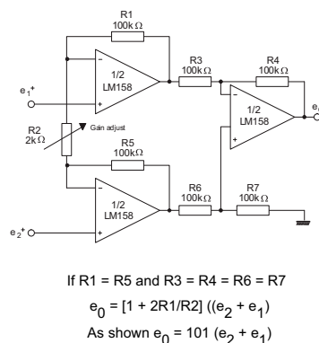
Figure 23. High input Z adjustable gain DC instrumentation amplifier
