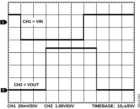
Figure 18. Propagation Delay Timing, 10 mV Overdrive
