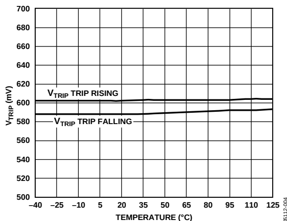
Figure 5. V_{IN} Trip Threshold vs. Temperature ( V_{CC} = 3.3 V)
