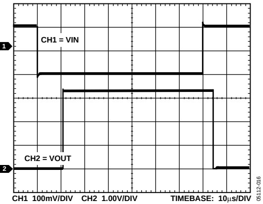
Figure 19. Propagation Delay Timing, 100 mV Overdrive
