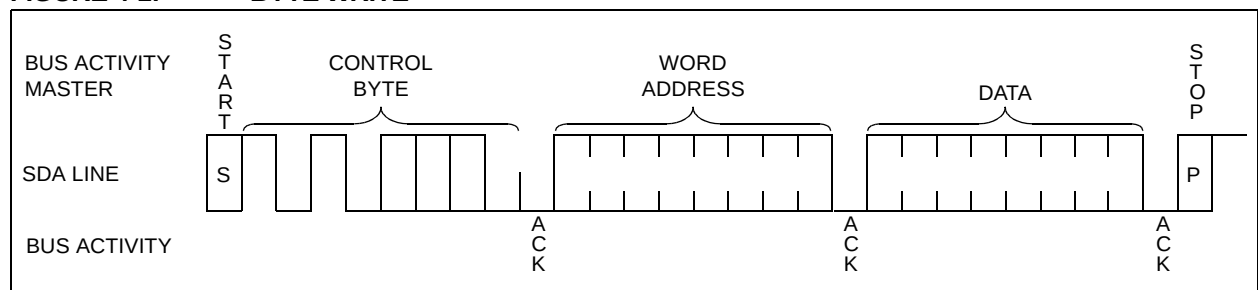
FIGURE 4-1: BYTE WRITE
