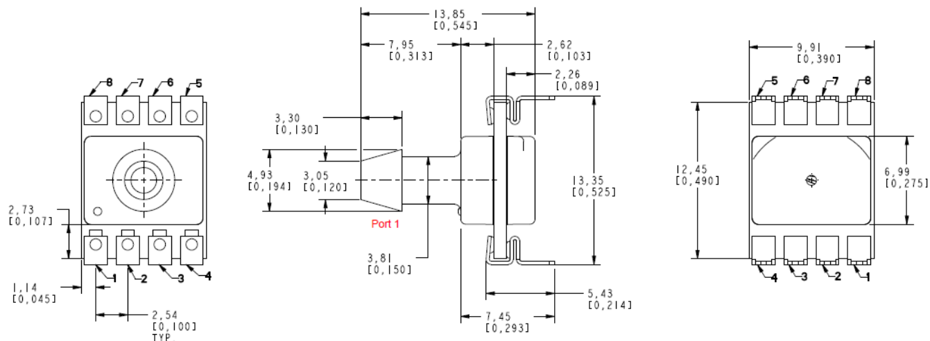
Figure 4. Package Dimensional Drawings (continued)
