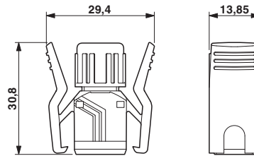
RJ45 sleeve housing, IP20, turned
