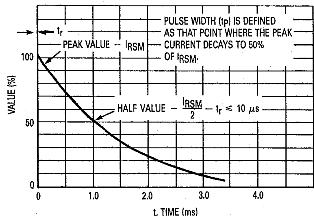
Figure 2. Pulse Waveform
