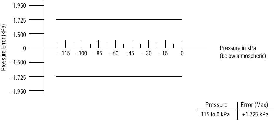
Pressure Error Band
