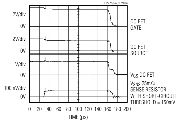
SHORT-CIRCUIT PROTECTION DELAY
