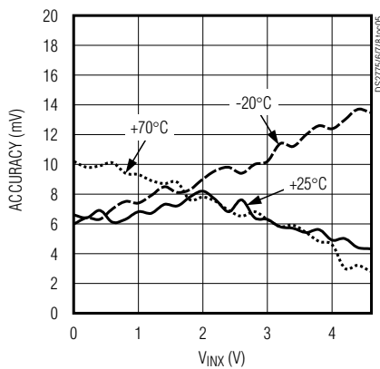
VOLTAGE MEASUREMENT ACCURACY
