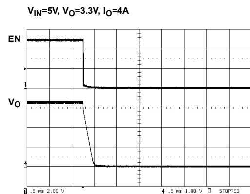
FIGURE 19. SHUT-DOWN
