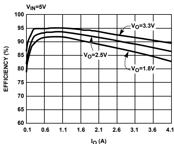
FIGURE 2. EL7564CRE EFFICIENCY
