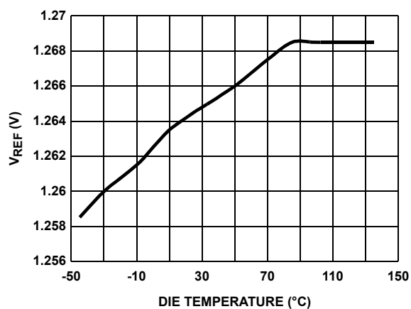
FIGURE 13. V_{REF} vs DIE TEMPERATURE
