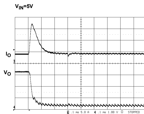
FIGURE 20. SHORT-CIRCUIT PROTECTION
