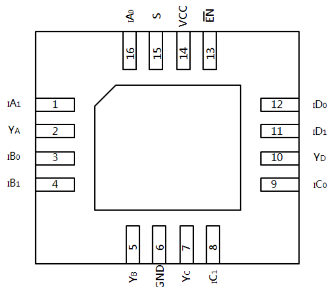
UQFN3x3-16 Top View
