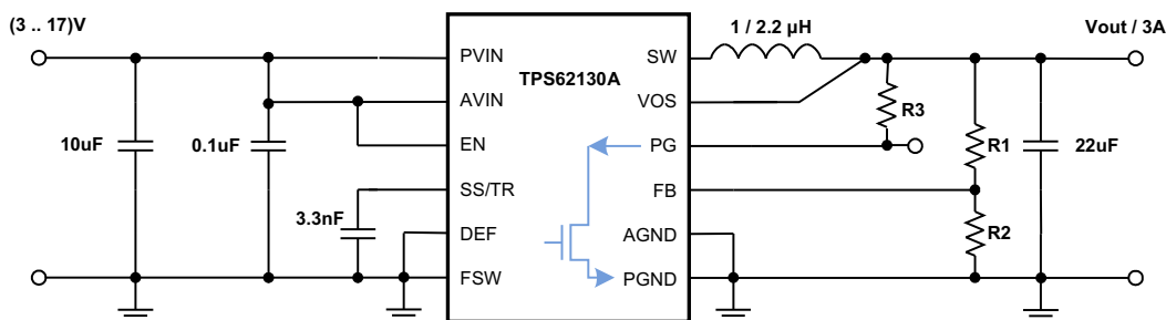
Figure 9-41. Discharge V OUT Through PG Pin with TPS62130A
