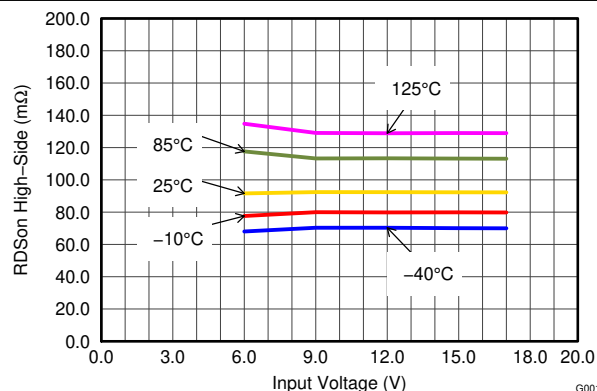
Figure 7-3. High-Side Switch Resistance
