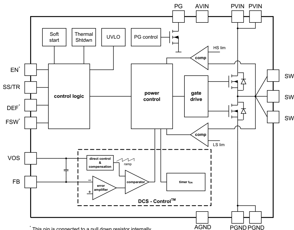
Figure 8-1. TPS62130 and TPS62130A (Adjustable Output Voltage)
