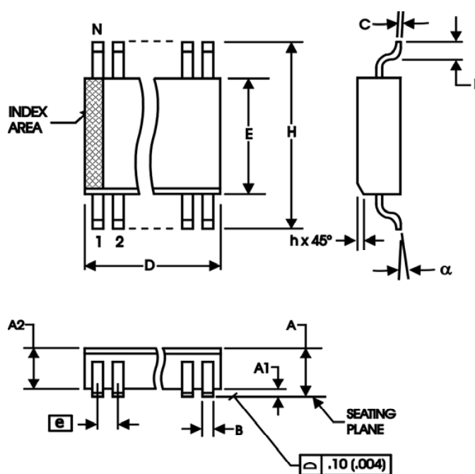
PACKAGE OUTLINE - M SUFFIX FOR 20 LEAD SOIC
