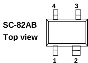
Figure 3 SC-82AB
