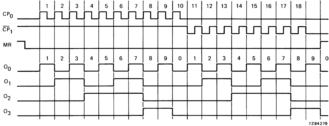
Fig.6 Timing diagram.
