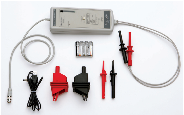
Figure 3. N2891A 70-MHz high-voltage differential probe with standard accessories.
