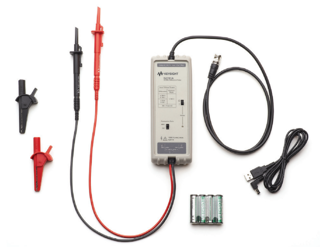
Figure 2. N2791A 25-MHz high-voltage differential probe with standard accessories
