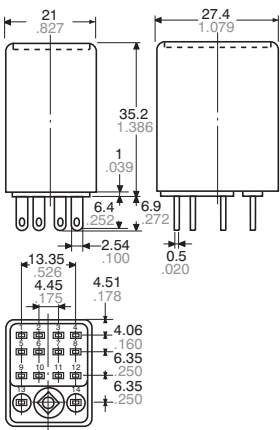
External dimensions
