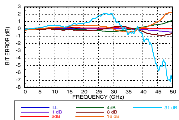
Bit Error vs. Frequency
