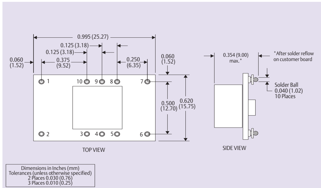
Figure 10 - Surface-Mount
