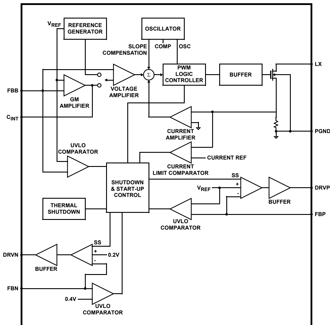
FIGURE 17. BLOCK DIAGRAM
