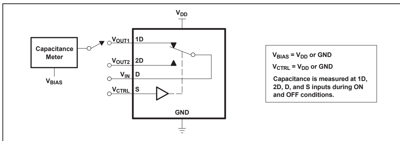
Figure 10. Capacitance
