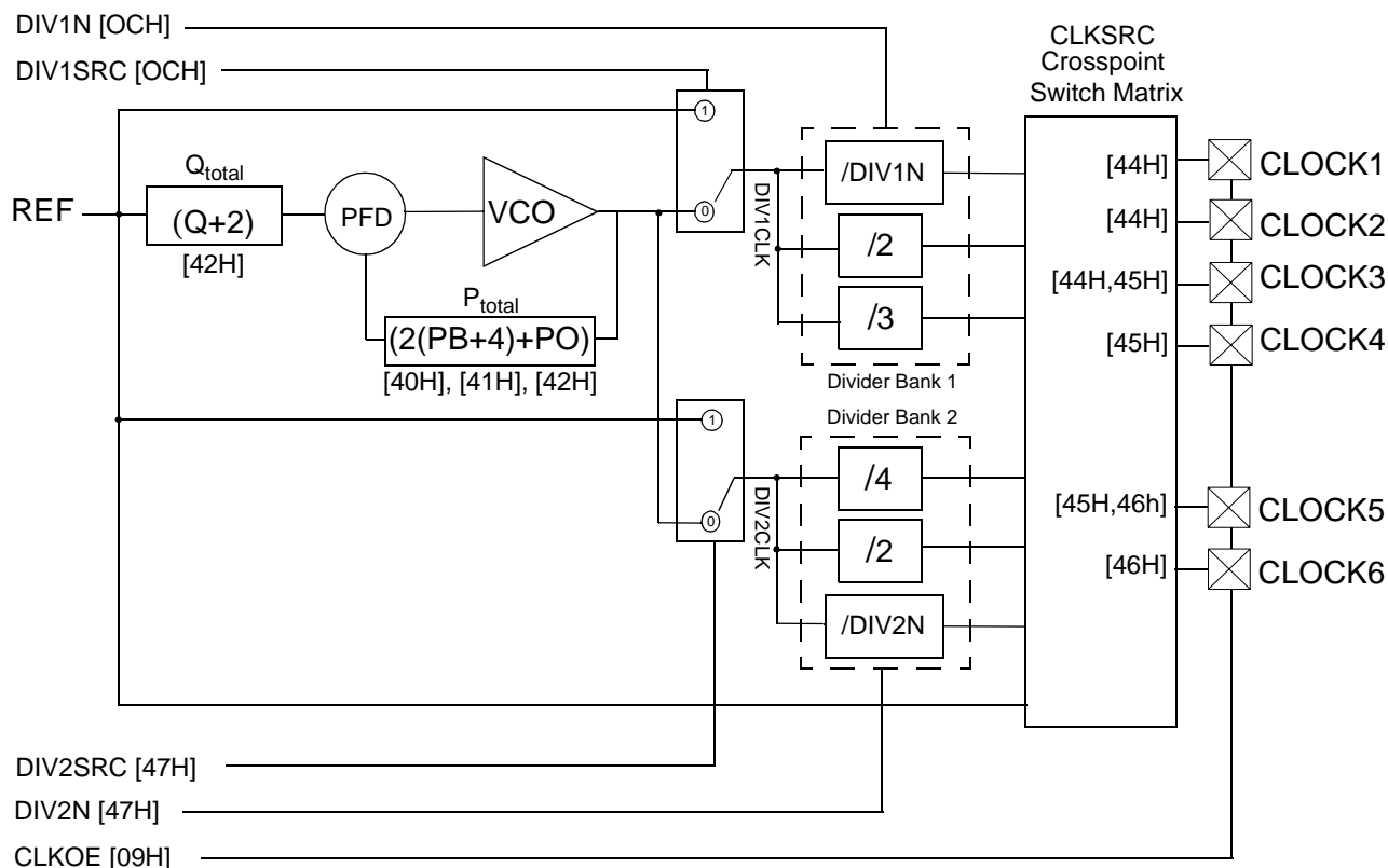
Figure 2. Basic Block Diagram of CY27EE16ZE PLL
