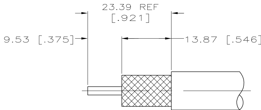
VIEW Z RECOMMENDED STRIP LENGTH SCALE 2:1
