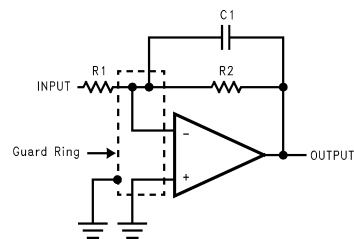
Inverting Amplifier
