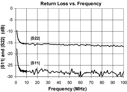
Typical 5-100 MHz RF Performance: V s =8V, I D =150mA @ T L =+25°C, Push-Pull Configuration
