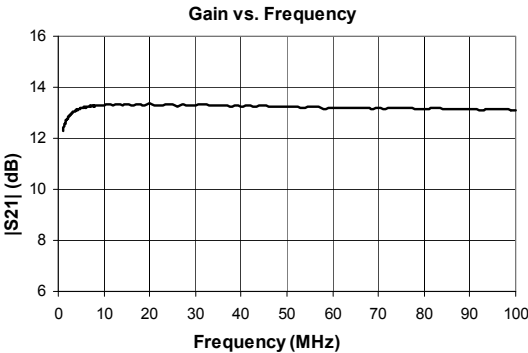
Typical 5-100 MHz RF Performance: V s =8V, I D =150mA @ T L =+25°C, Push-Pull Configuration
