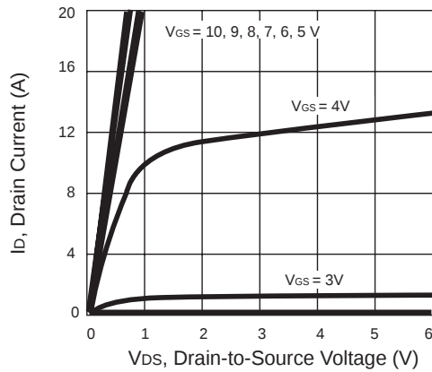
Figure 1. Output Characteristics
