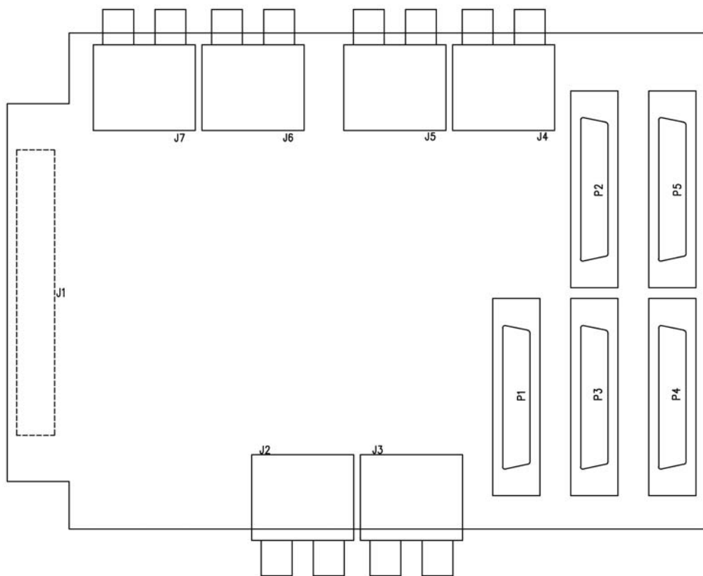
Figure 2-5. Connector Locations
