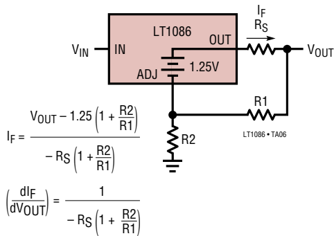
Battery Charger
