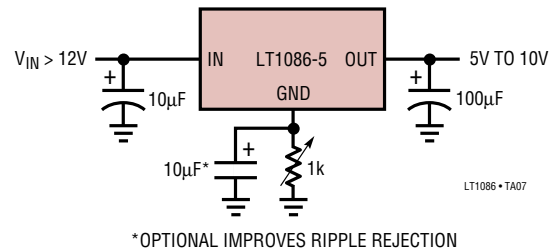
Adjusting Output Voltage of Fixed Regulators
