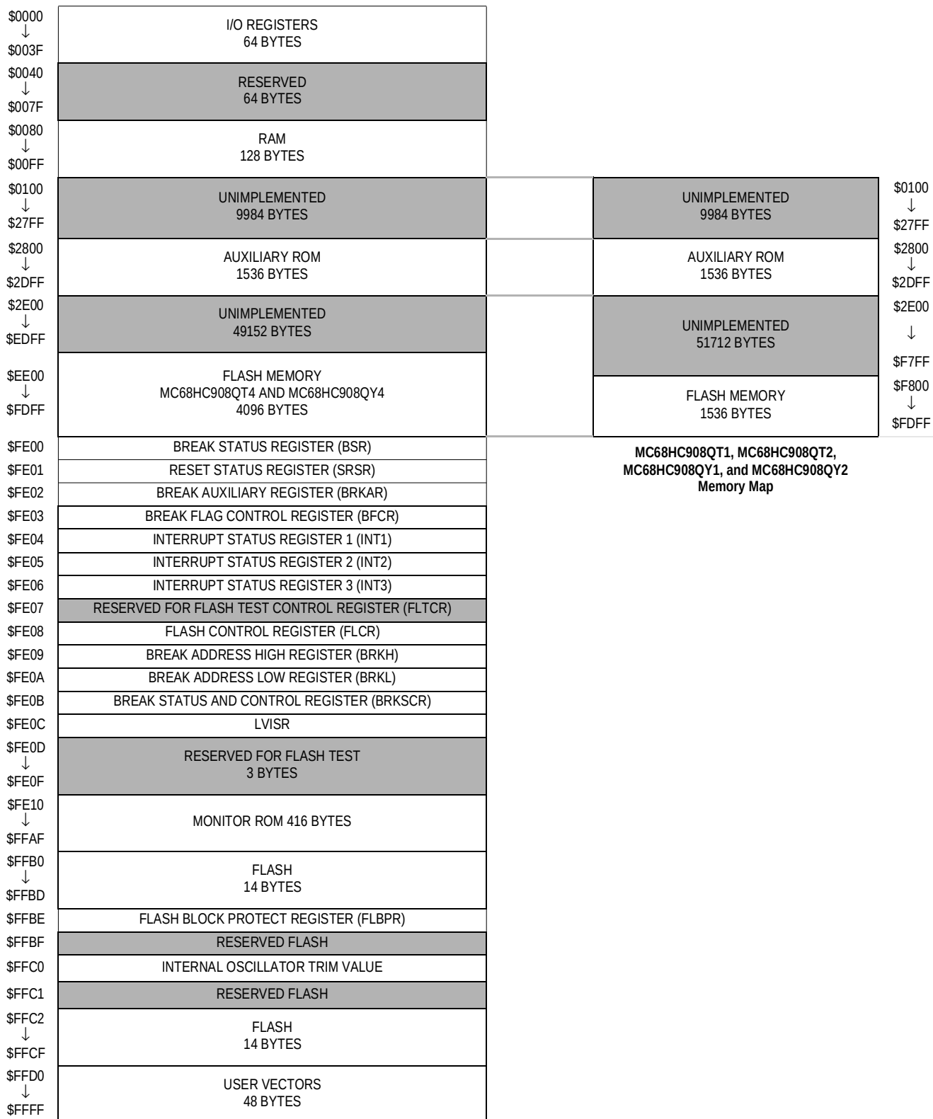
Figure 2-1. Memory Map
