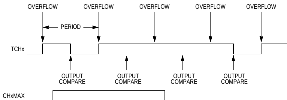
Figure 10-8. CHxMAX Latency
