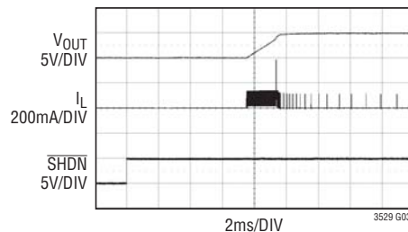
Soft-Start Waveforms
