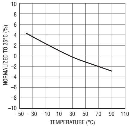
Switching Frequency Variation vs Temperature
