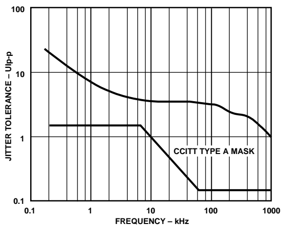
Figure 5. Jitter Tolerance
