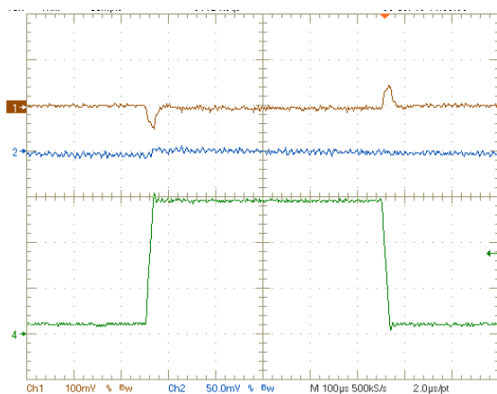
FIGURE 9. DCD1 TRANSIENT RESPONSE ( V_{IN} = 3.6V , STEP LOAD: 150mA TO 1500mA) CH1: VODCD1 (100mV/DIV, AC), CH2: VODCD2 (50mV/DIV, AC), CH4: IL4 (500mA/DIV)
