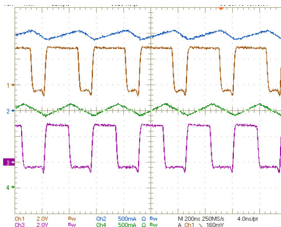
FIGURE 8. INDUCTOR CURRENT RIPPLE ( V_{IN} = 3.6V , FULL LOADING, PWM, TIME SCALE = 200ns) CH1: SW1 (2V/DIV), CH2: IL1 (500mA/DIV), CH3: SW2 (2V/DIV), CH4: IL2 (500mA/DIV)
