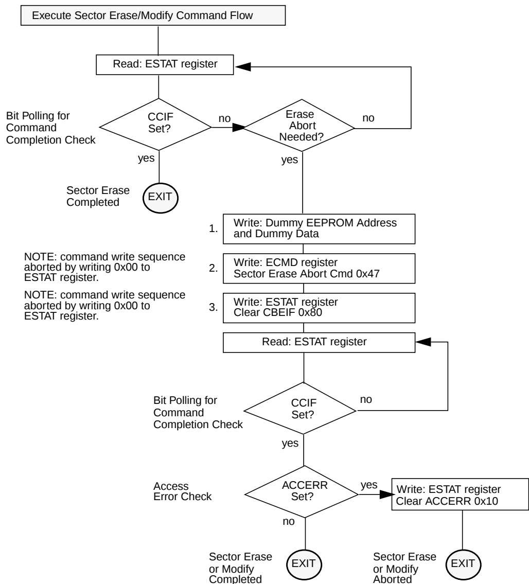
Figure 25-22. Example Sector Erase Abort Command Flow
