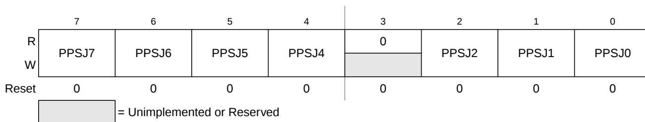
Figure 22-61. Port J Polarity Select Register (PPSJ)
