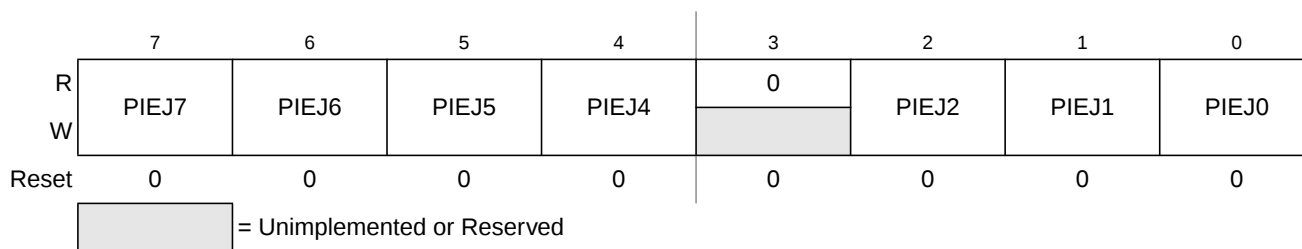
Figure 22-62. Port J Interrupt Enable Register (PIEJ)
