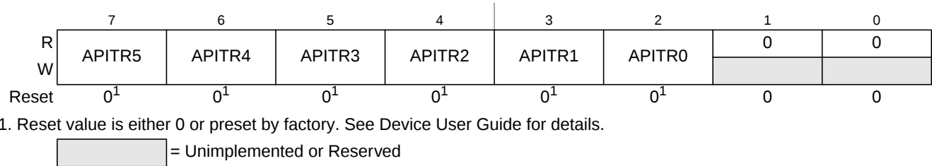
Figure 14-5. Autonomous Periodical Interrupt Trimming Register (VREGAPITR)
