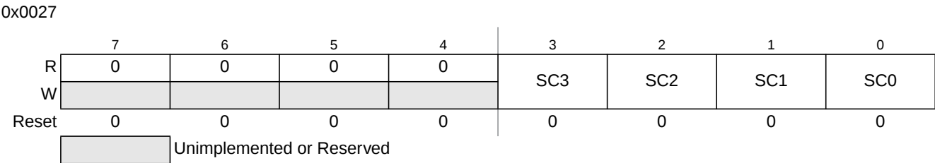
Figure 19-12. Debug State Control Register 3 (DBGSCR3)
