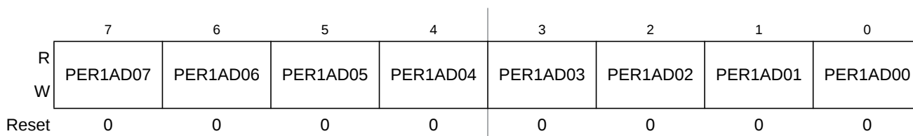
Figure 23-67. Port AD0 Pull Up Enable Register 1 (PER1AD0)
