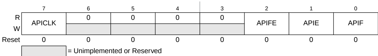
Figure 14-4. Autonomous Periodical Interrupt Control Register (VREGAPICL)
