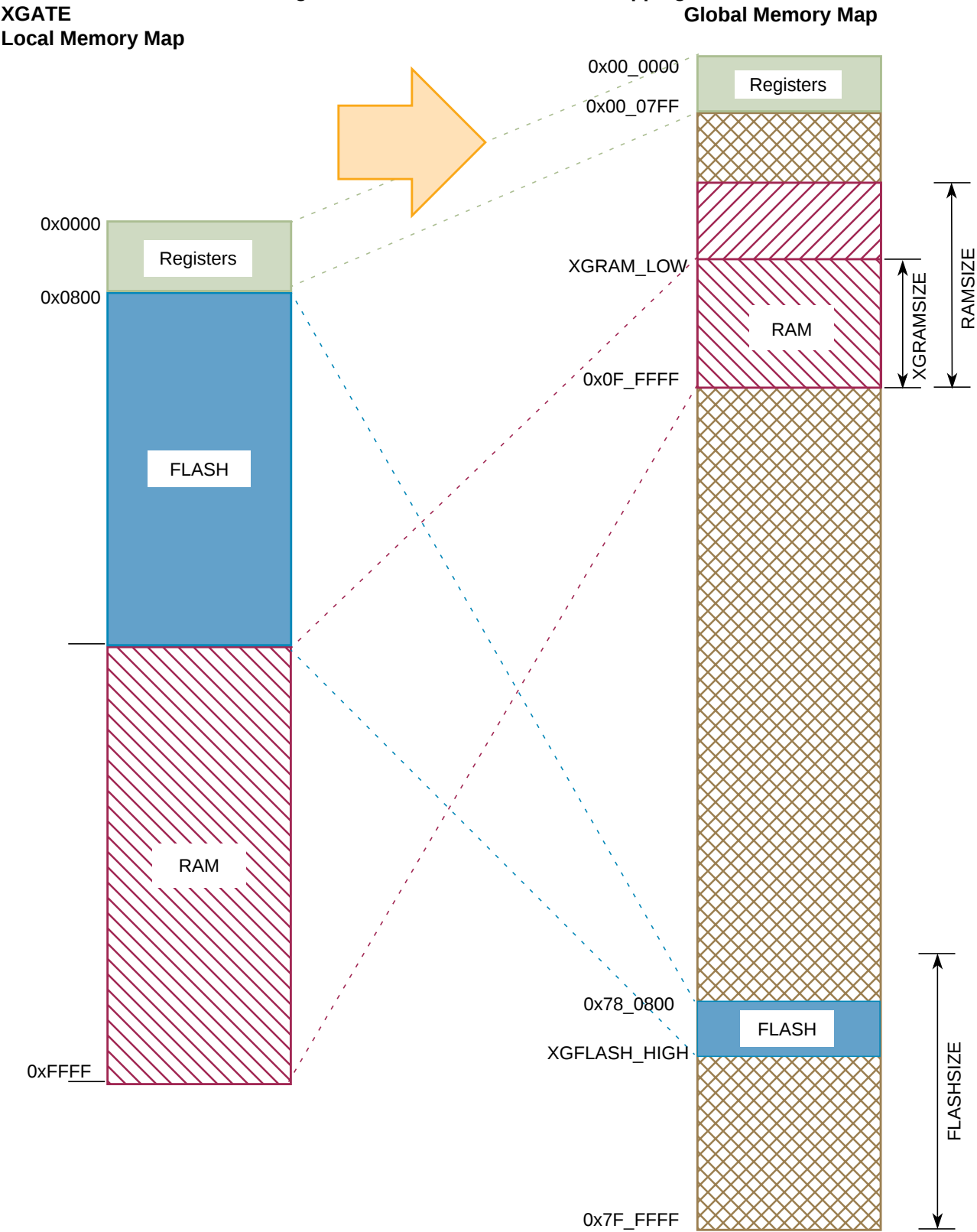
Figure 1-5. GATE Global Address Mapping
