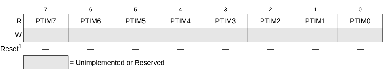
Figure 22-33. Port M Input Register (PTIM)
