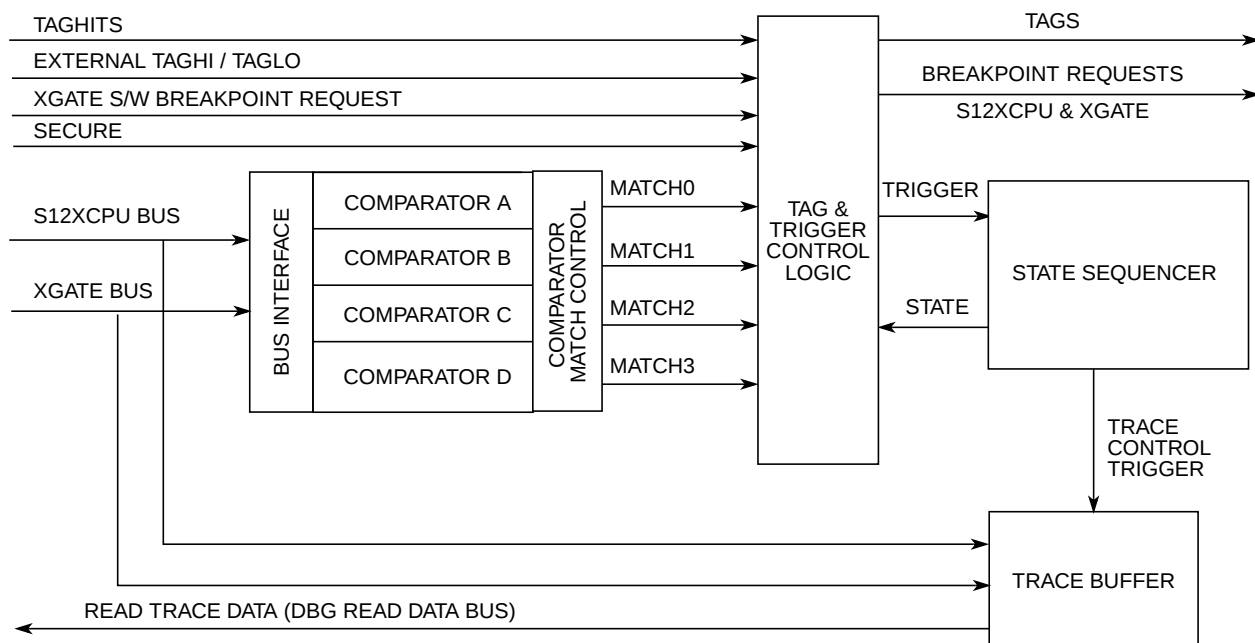
Figure 20-22. S12XDBG Overview
