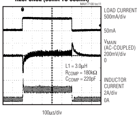
STEP-UP REGULATOR LOAD-TRANSIENT RESPONSE (50mA TO 500mA)
