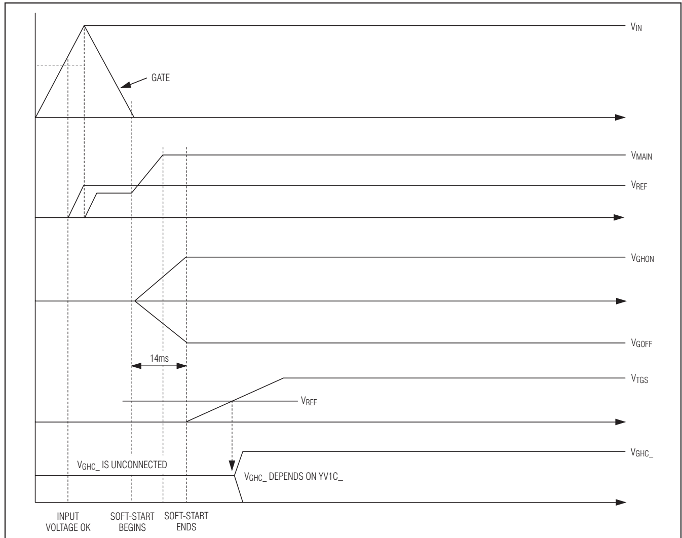
Figure 7. Power-Up Sequence
