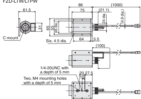
High-luminance Pattern Lighting FZD-LTW/LTPW
