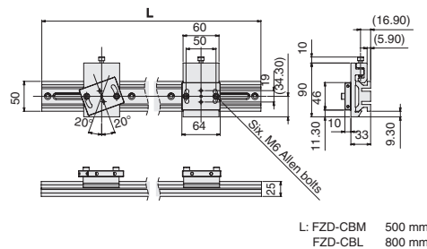
3D Camera Base FZD-CBM/CBL
