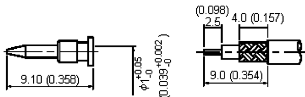
Stripping Dimension
