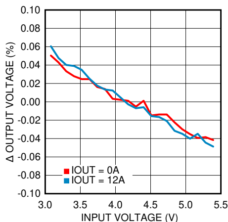
Figure 8-11. Line Regulation
