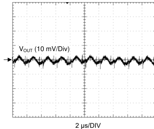
Figure 8-13. Output Voltage Ripple (I OUT = 15 A)
