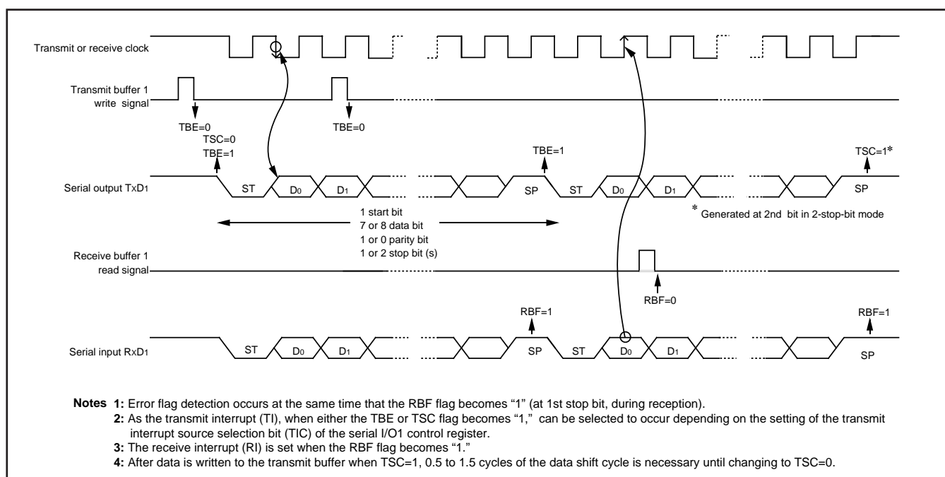
Fig. 51 Operation of UART serial I/O function
