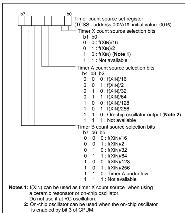
Fig. 26 Timer count source set register
