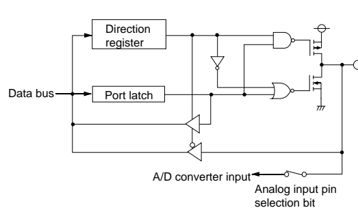
(13) Ports P20–P27
