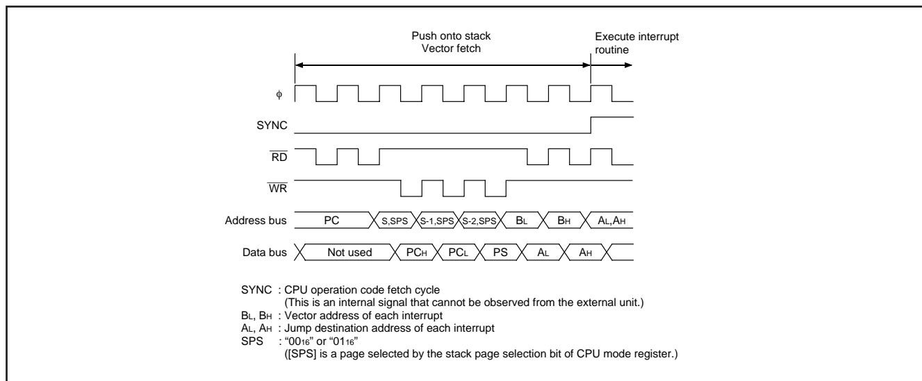
Fig. 19 Interrupt sequence
