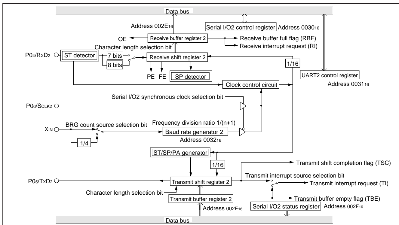
Fig. 58 Block diagram of UART serial I/O2
