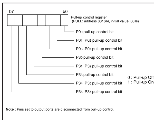
Fig. 11 Structure of pull-up control register
