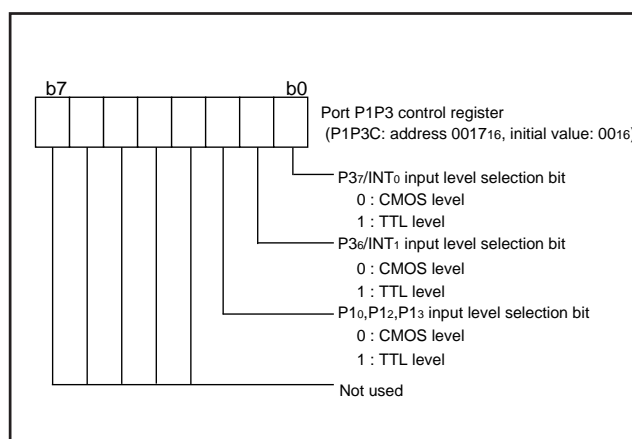
Fig. 12 Structure of port P1P3 control register
