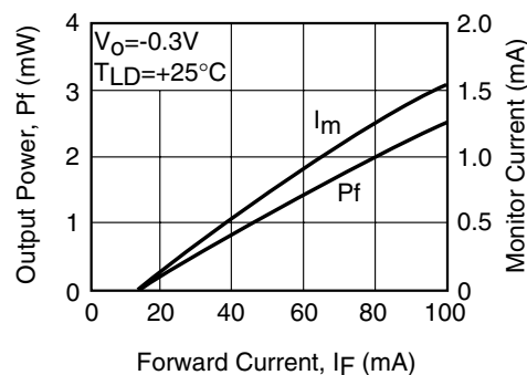
Fig. 2 Output Power & Monitor Current vs. Forward Current
