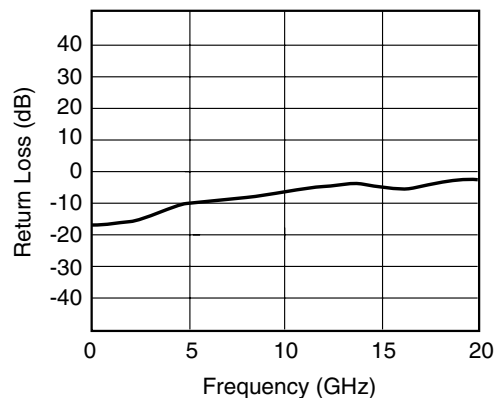
Fig. 5 RF Return Loss (S11)
