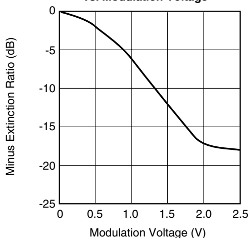
Fig. 3 Extinction Ratio vs. Modulation Voltage
