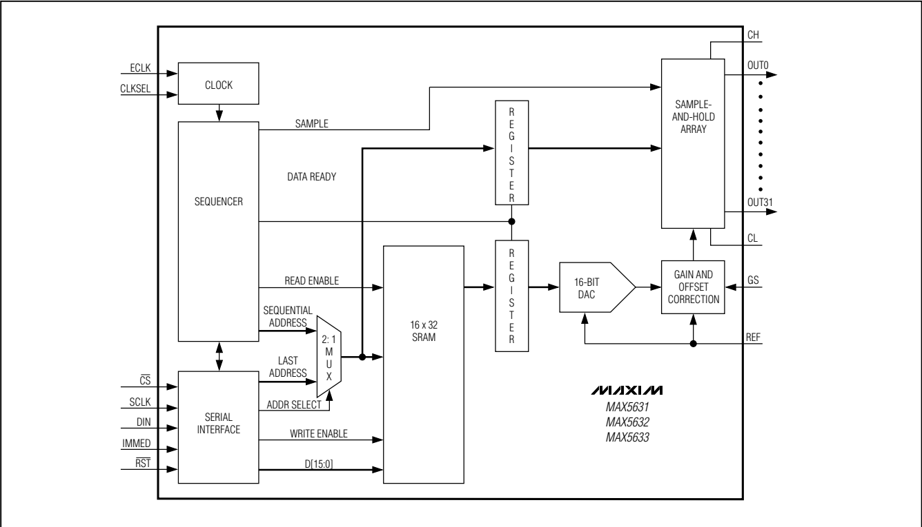
Figure 1. Functional Diagram
