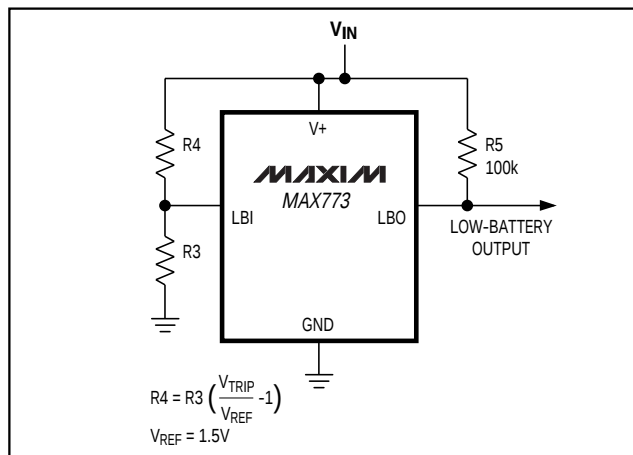
Figure 9. Input Voltage Monitor Circuit
