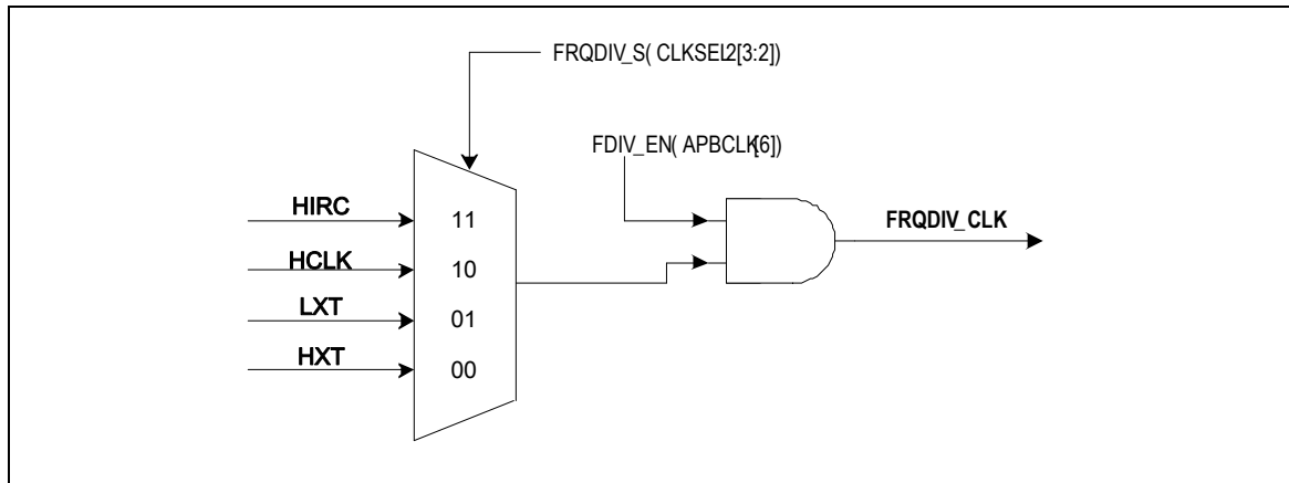
Figure 5-3 Clock Sources of Frequency Divider
