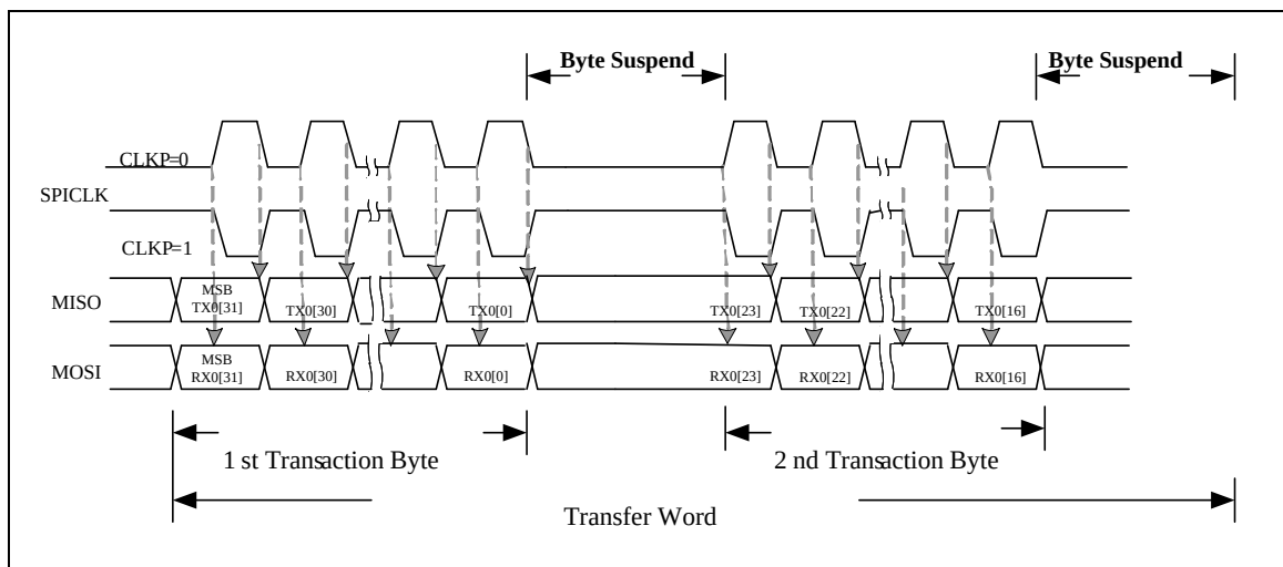
Figure 5-97 SPI Byte Suspend Mode
